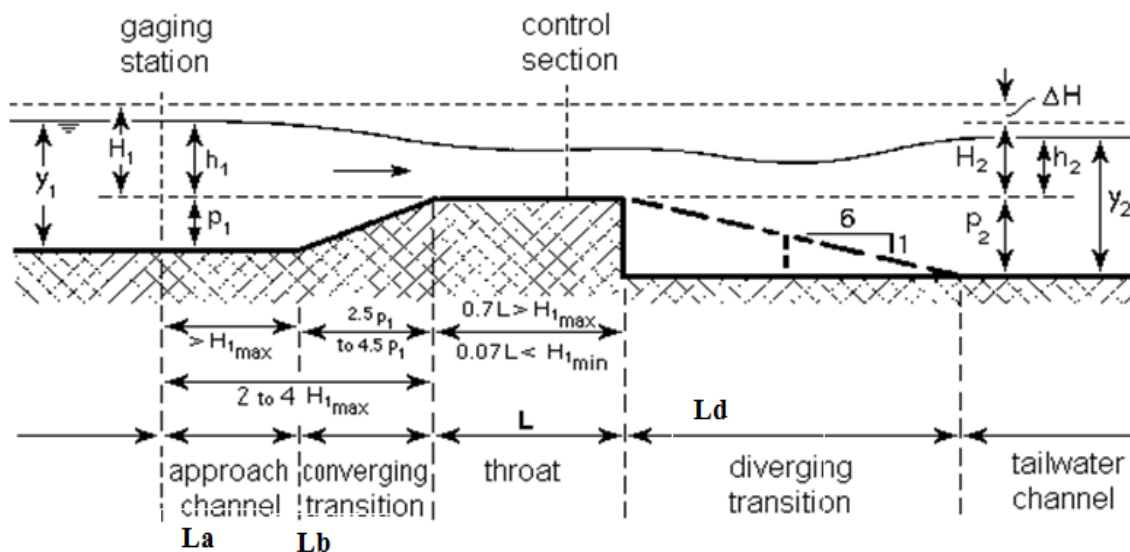
Figure 1: Side view of a long through flume
