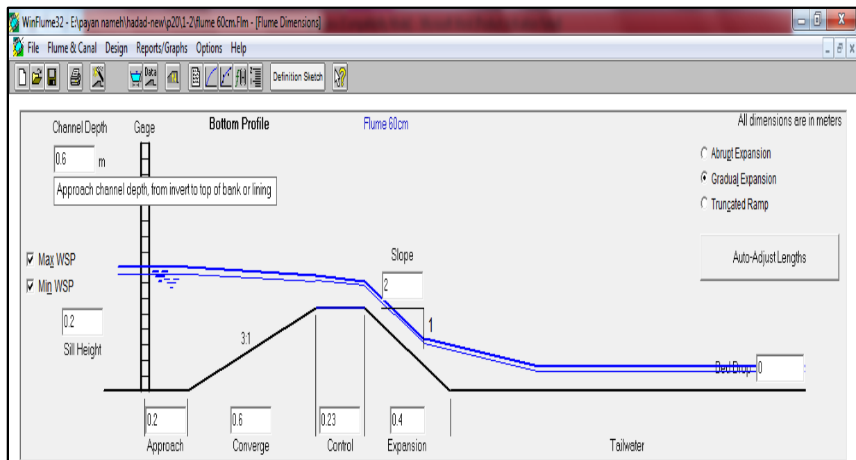
Figure 2: Long throat flume design with 20 cm sill height and 1:2 slope (WinFlume)
