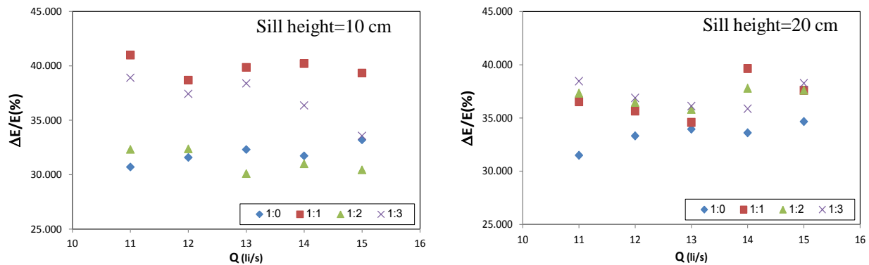
Figure 6: Energy depreciation in Different sill height and slope
