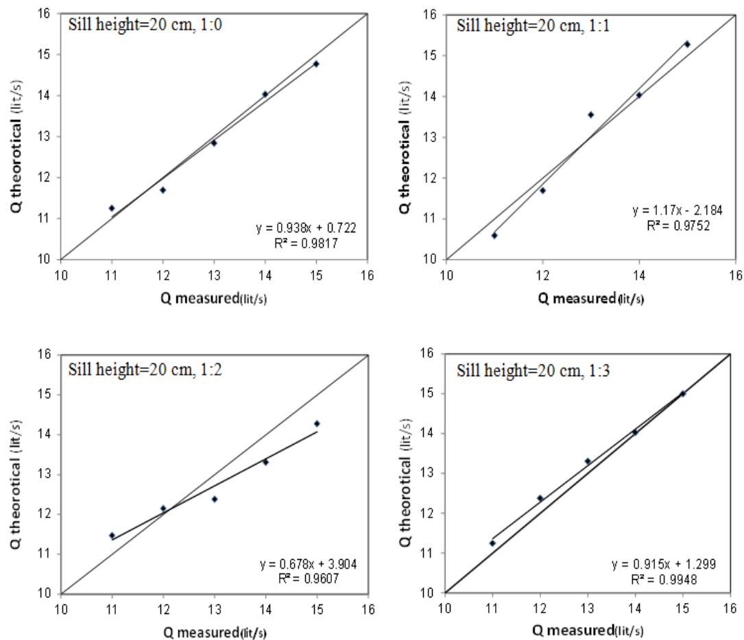
Figure 5: Q-theoretical and Q-measured relationship in long throat flume with 20 cm sill height
