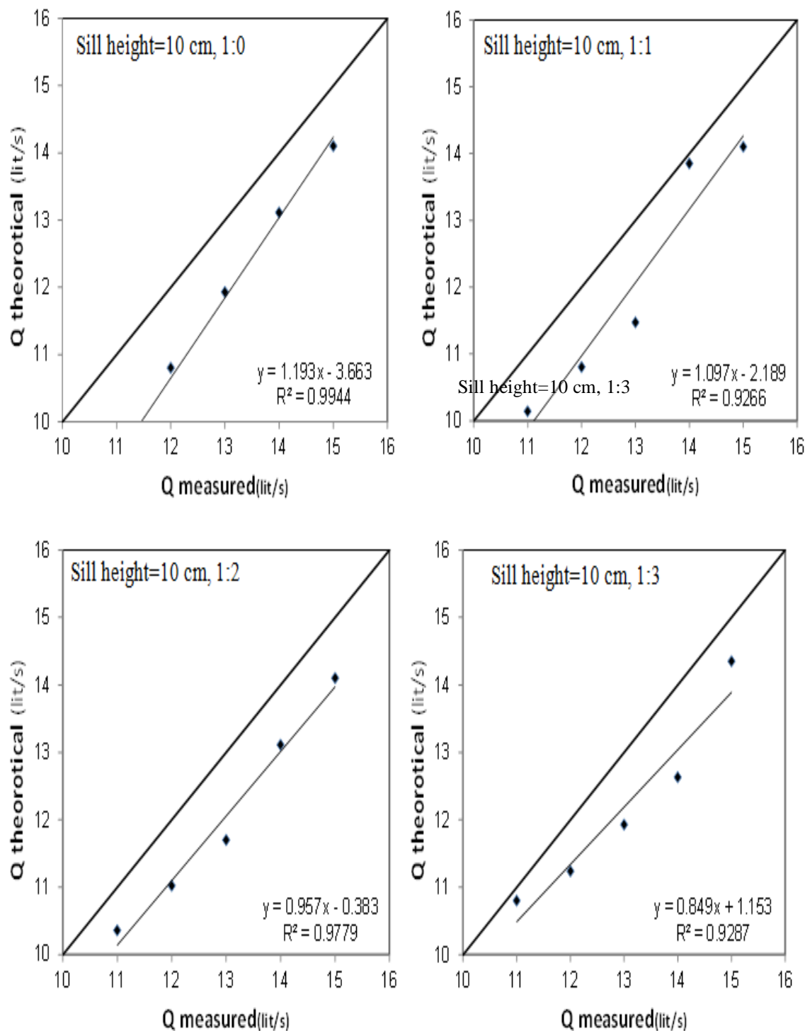
Figure 4: Q-theoretical and Q-measured relationship in long throat flume with 10 cm sill height
