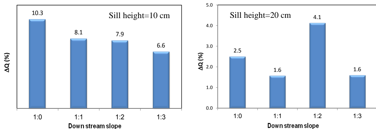
Figure 4: Difference between measured discharges and theoretical discharges
